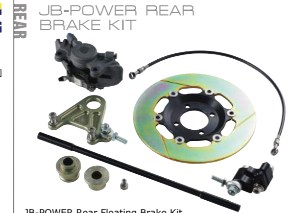
JB-POWER Rear Floating Brake Kit [Cast Iron Disc φ250, CP2696 Caliper, Brake Pads, Caliper Bracket [Collar included], Torque Rod, Torque Rod Anker, Stainless Mesh Brake Hose, Stainless Fitting, Banjo Bolt] ¥ 184,600.-
